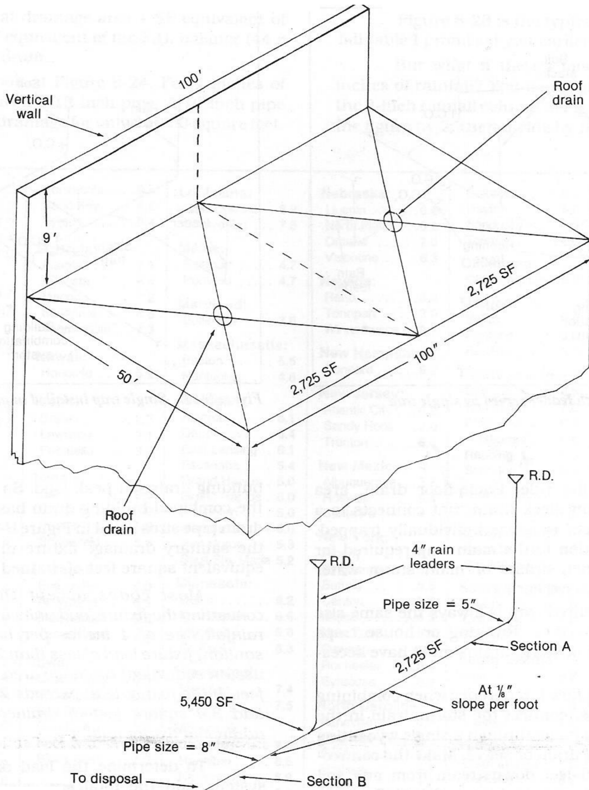
Figure 8-25 Storm water drainage system
